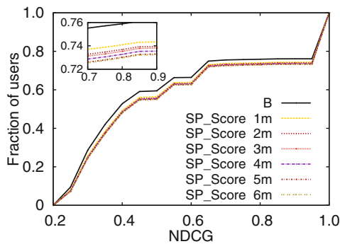
(c) NDCG distribution (SP_Score).
