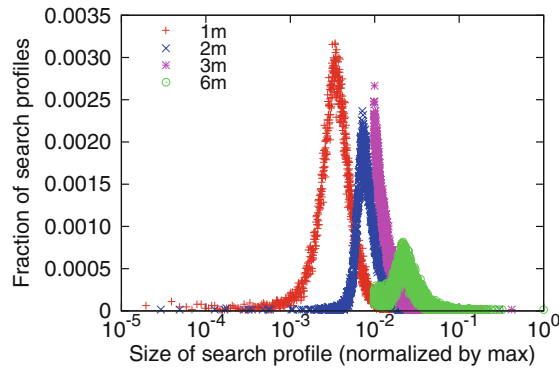
Fig. 6. Distribution of profile size.
