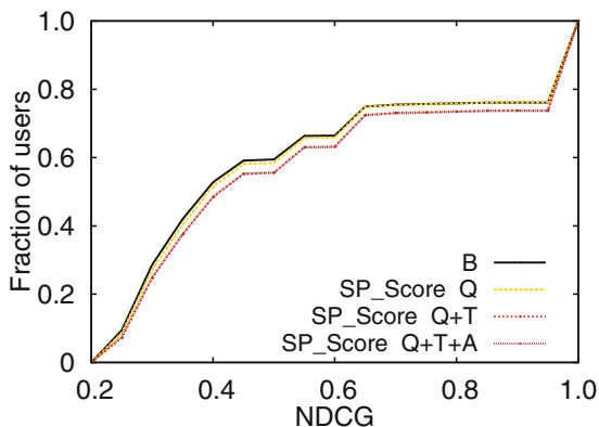
(b) NDCG distribution (SP_Score).
