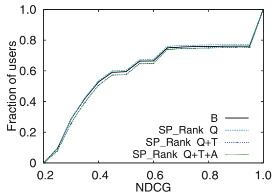
(c) NDCG distribution (SP_Rank).
