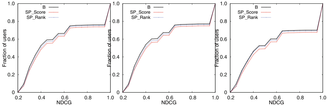
(b) NDCG distribution: all users (left), active users (middle), inactive users (right)
